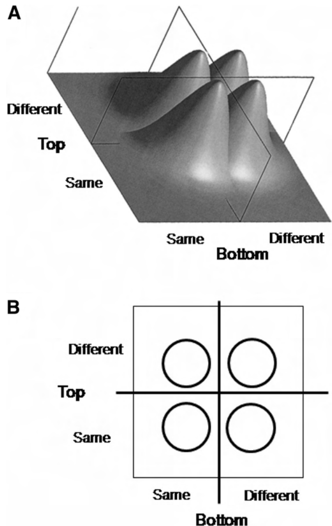
Figure 1. Example of a representation of the four stimuli in a sequential matching task in three-dimensional perceptual space. A: Bivariate normal probability distributions of perceptual effects for each of the four stimuli and decision boundaries. B: The contours of equal likelihood for these distributions, which are created by slicing each distribution along an equal plane and then viewing the sliced distributions from above.
